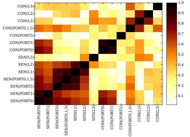
Figure 7. The absolute values of Pearson correlation coefficient among all the sensitivity and contentiousness dimensions. 97.96% of the pairs have a correlation coefficient lower than 0.80 and the majority of the pairs, lower than 0.50.
